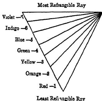
Fig 33 PRISMATIC SPECTRUM
